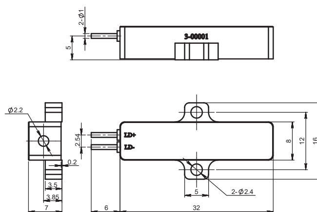
F3A Drawing
