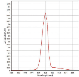
808nm Spectrum
