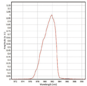
980nm Spectrum
