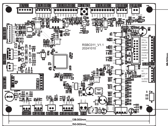
Control board
