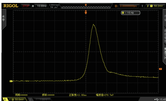
Typical Pluse
