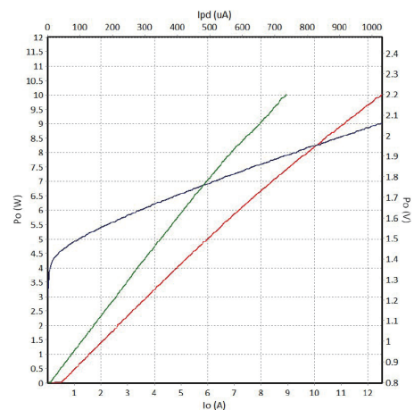
980nm P-I-V Graph
